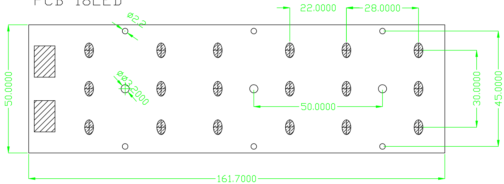
PCB 18LED
